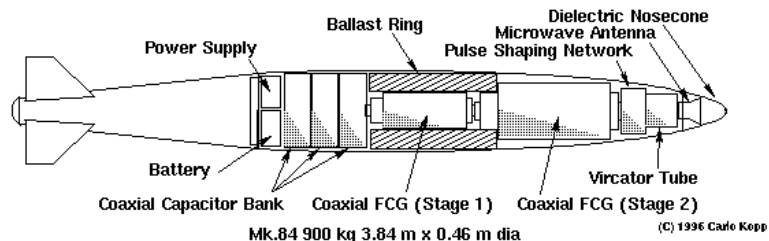
FIG.6 HPM E-BOMB WARHEAD (Mk.84 FORM FACTOR)
