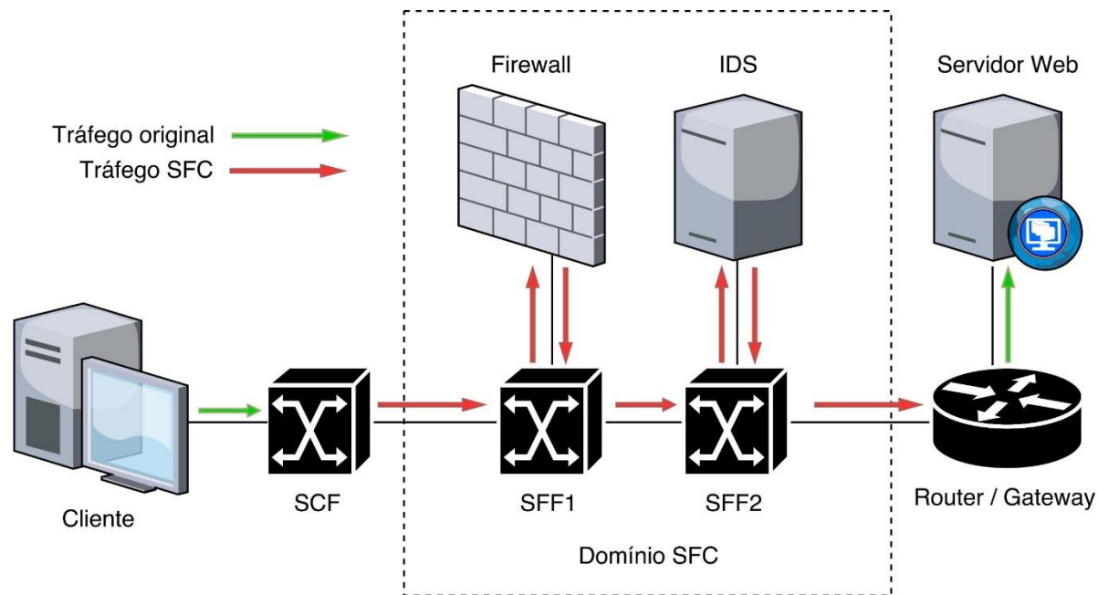
Service Function Chaining
